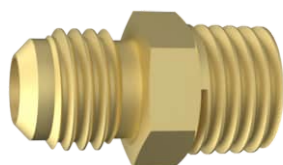
170400 | Rosca Externa: NPT 1/4" 170401 | Rosca Externa: NPT 3/8" 170402 | Rosca Externa: NPT 1/2"
