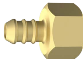
171000 Amarelo Saida Externa: TM 3/8" TERMINAL BSP X TM Rosca Externa: BSP 1/2" Material: Latão
